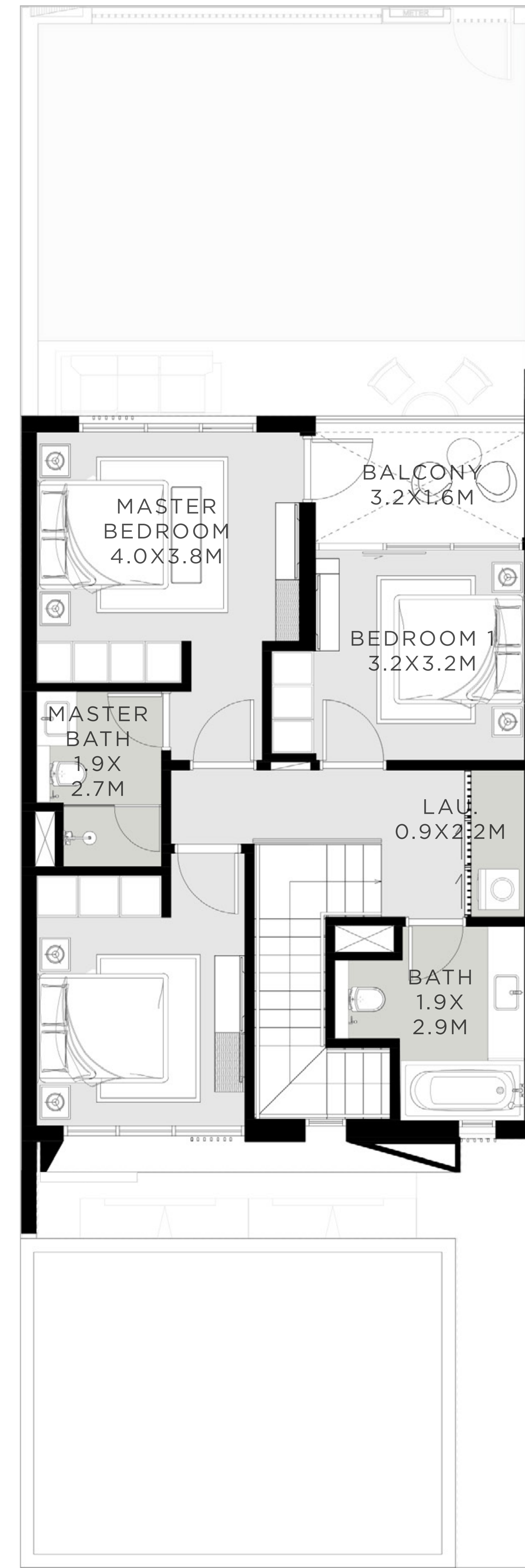
FIRST FLOOR
