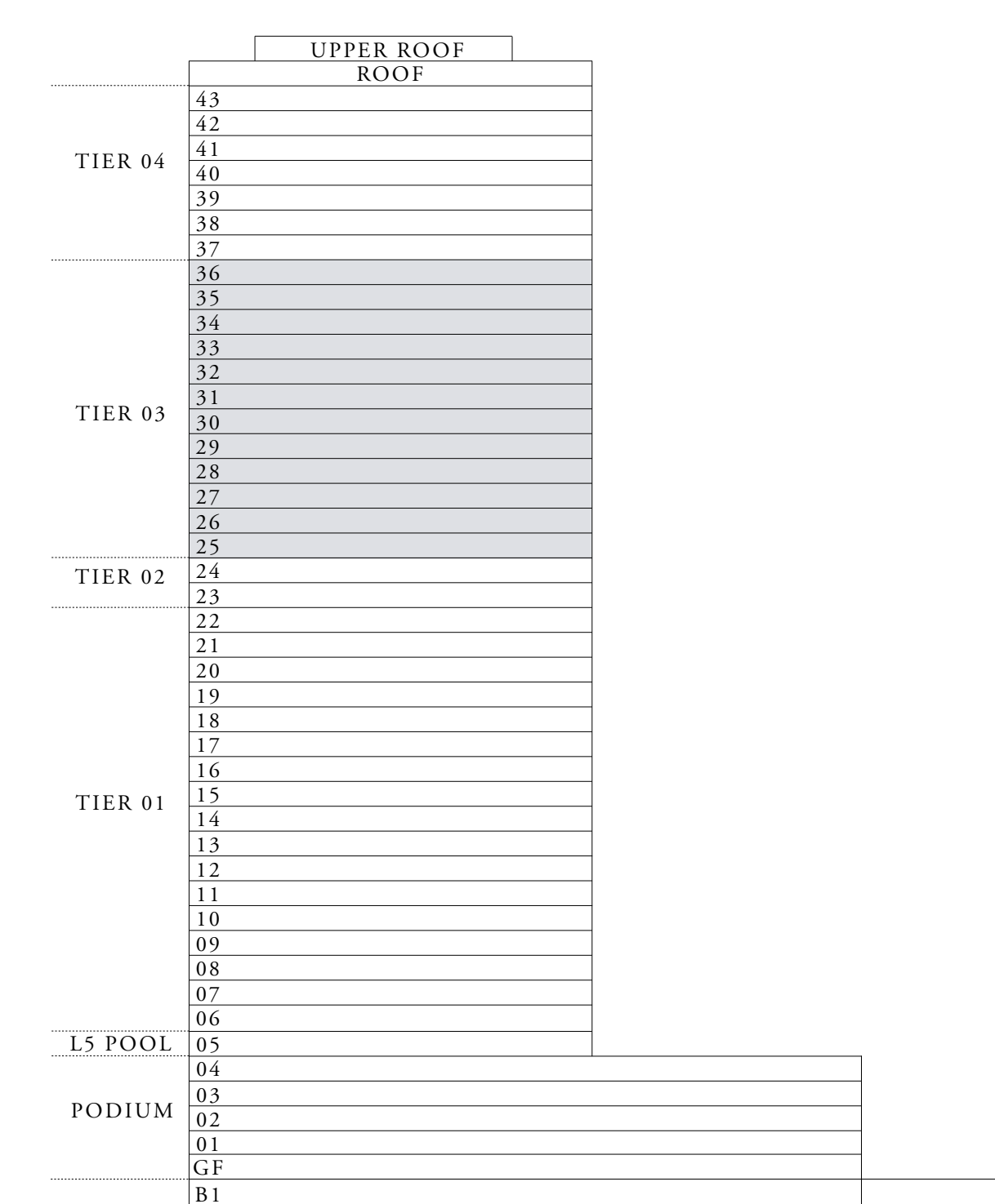
KEY SECTION
