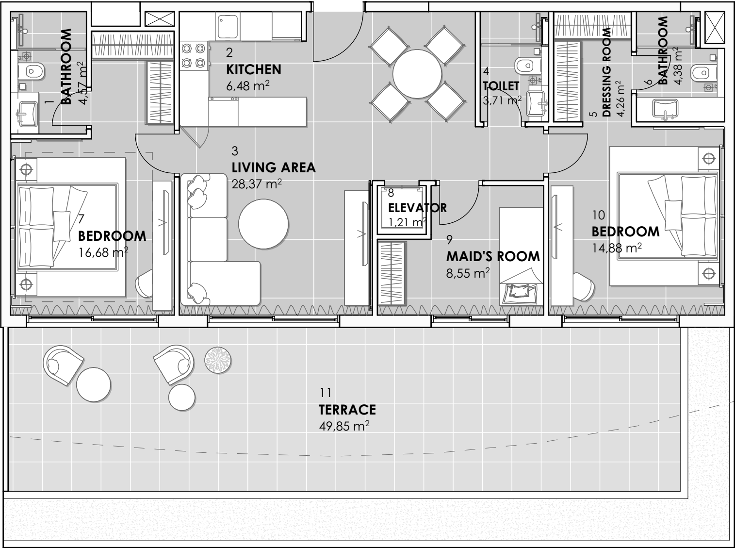
Roof terrace plan
